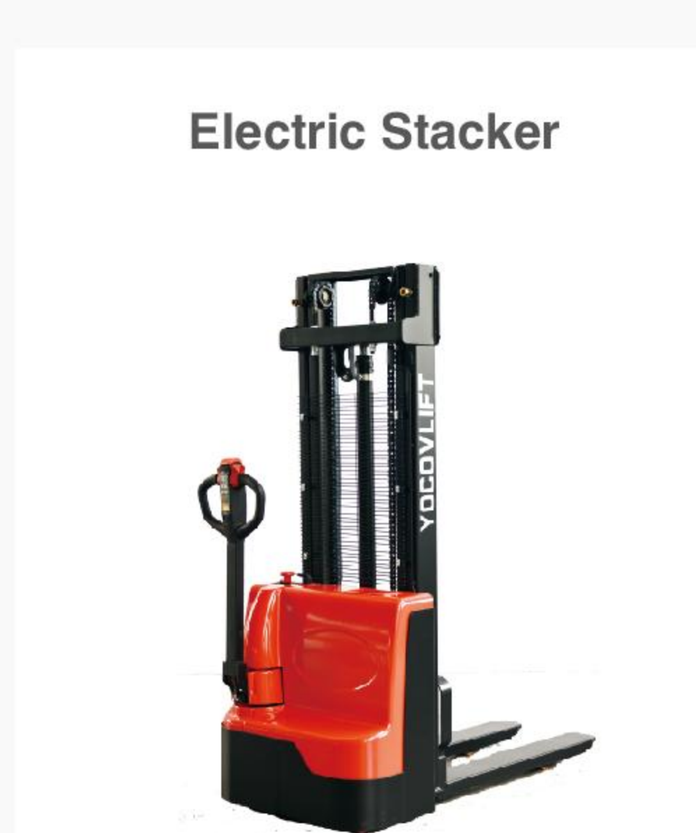
QES15E/QES20E Load Capacity: 1500/2000KG Lift Height: 1600~4000mm
