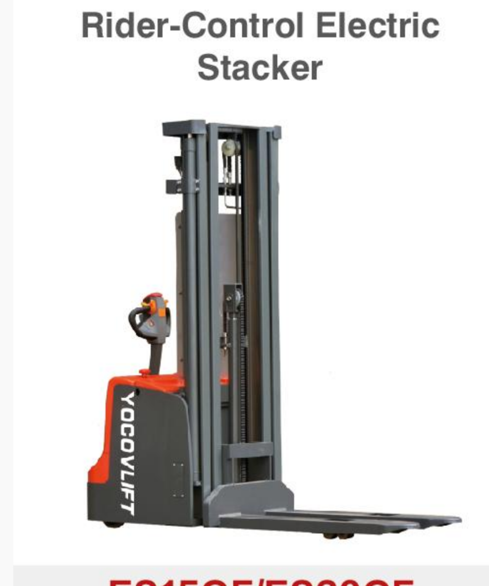
ES15GF/ES20GF Load Capacity: 1500/2000KG Lift Height: 3000~4500mm
