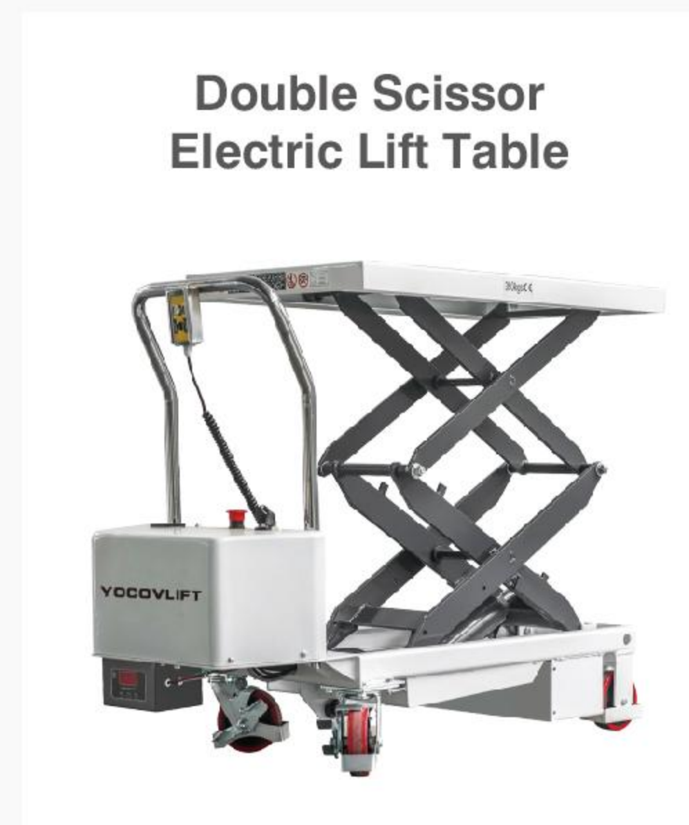
ETF30/35/50/75 Load Capacity: 300/350/500/750KG
