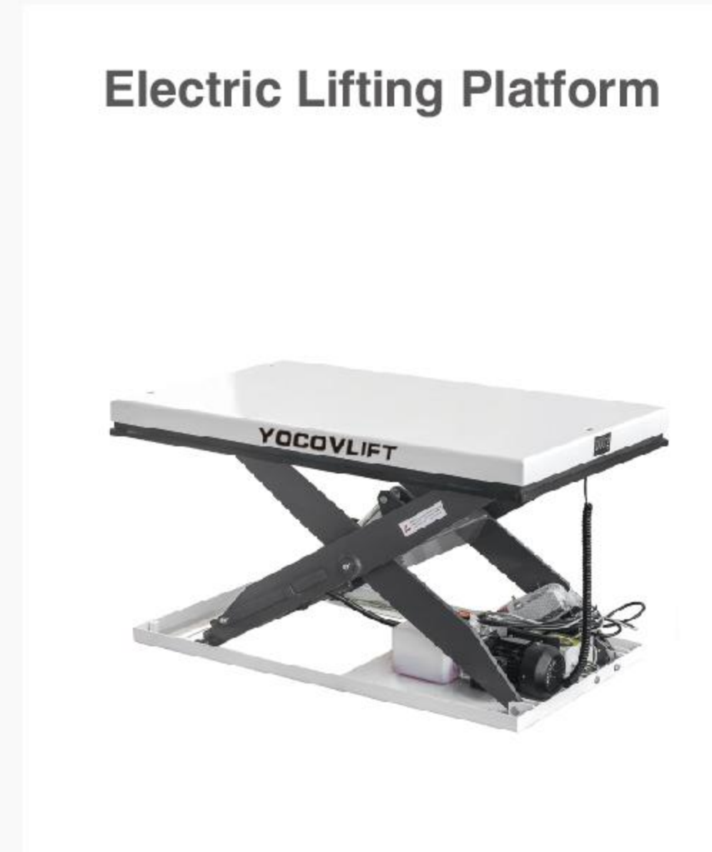
HIW1.0EU/2.0EU/3.0EU/4.0EU Load Capacity: 500/1000/2000/3000KG
