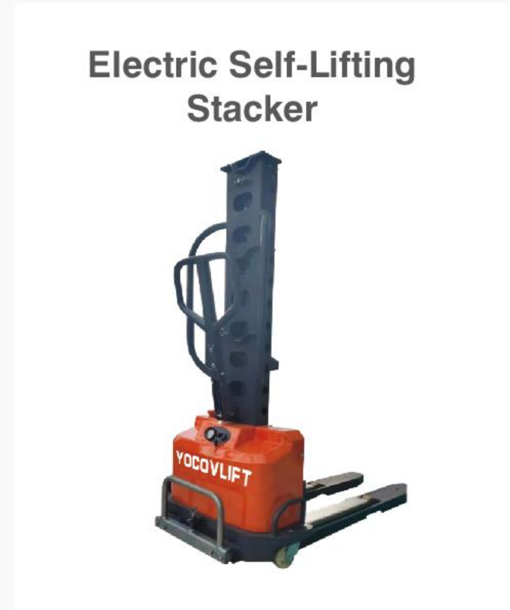
CDD05JZ Load Capacity: 500KG Max Lift Height: 1500mm
