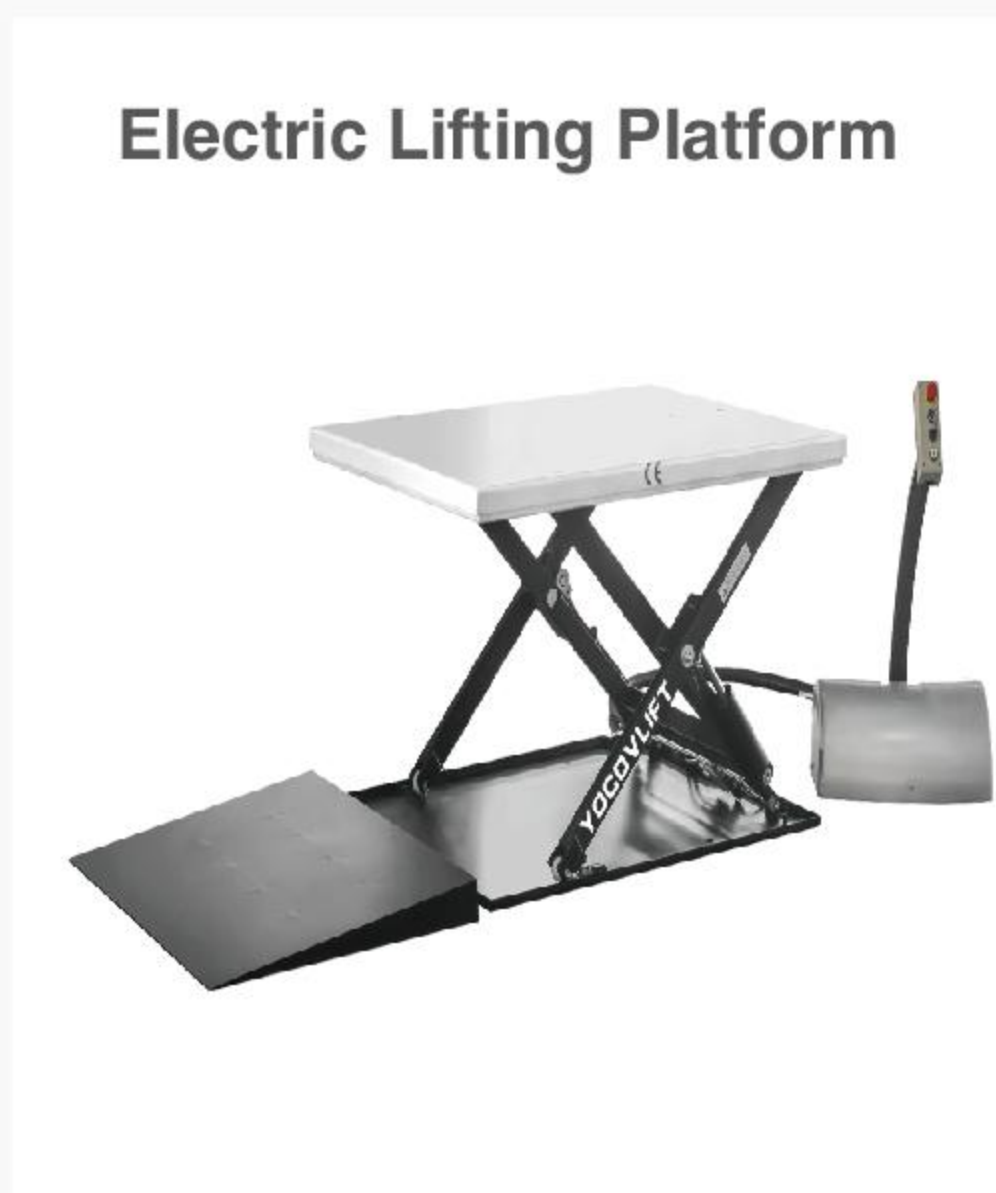
HTF-G05/G-10/G-20 Load Capacity: 500/1000/2000KG
