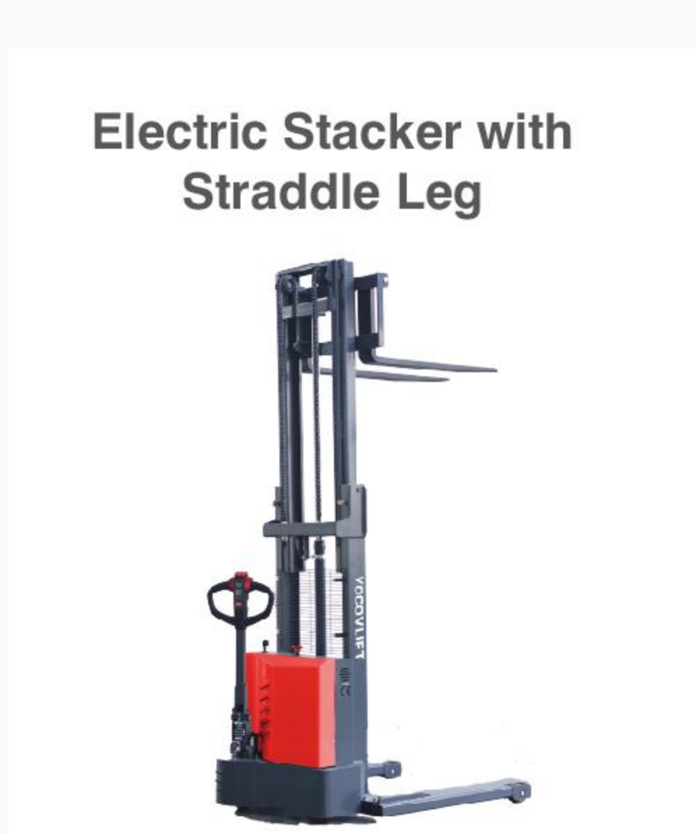
QES10E-SL/QES12E-SL Load Capacity: 1000/1200KG Lift Height: 1600~3500mm
