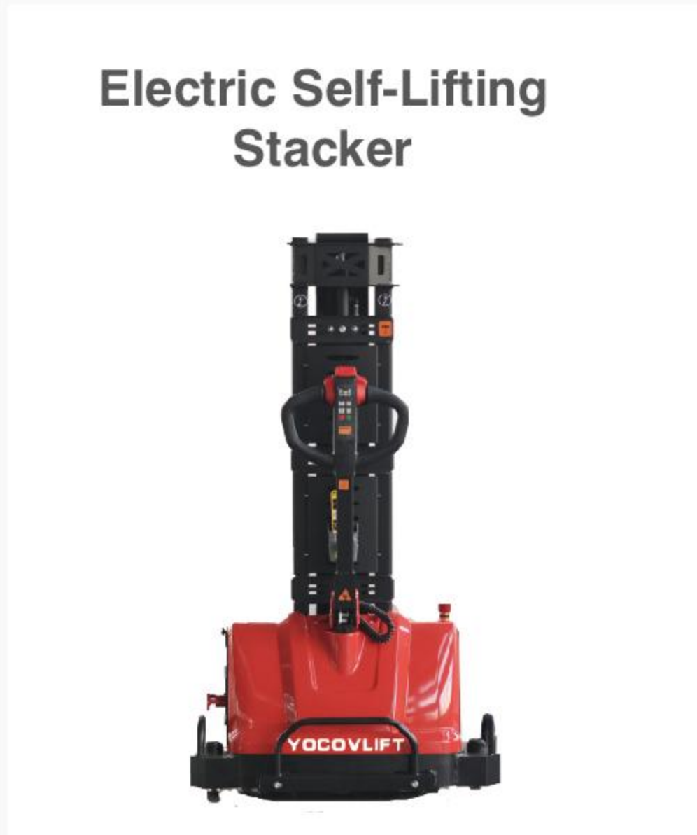
SES10/SES12 Load Capacity: 1000/1200KG Lift Height: 900~1600mm
